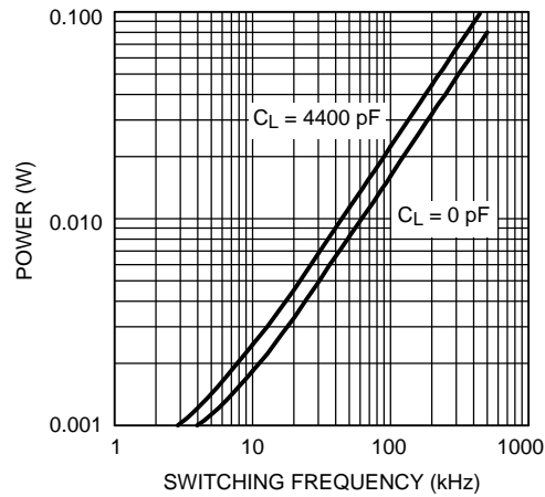
Figure 22. Diode Power Dissipation V_{IN} = 50V
